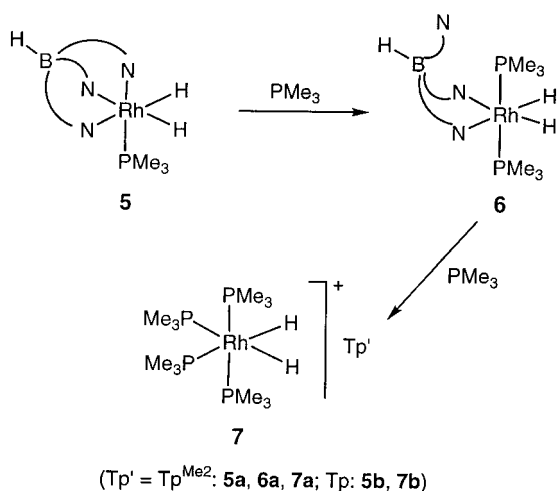
Scheme 2. Changes in the denticity of Tp and Tp Me2 in Rh III hydrido complexes. The reactions proceed at 50 °C for Tp' = Tp Me2 , and at room temperature for Tp' = Tp.
